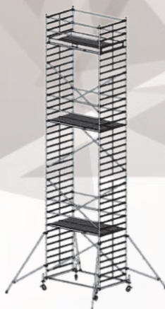
AS 4011 working height: 11m
